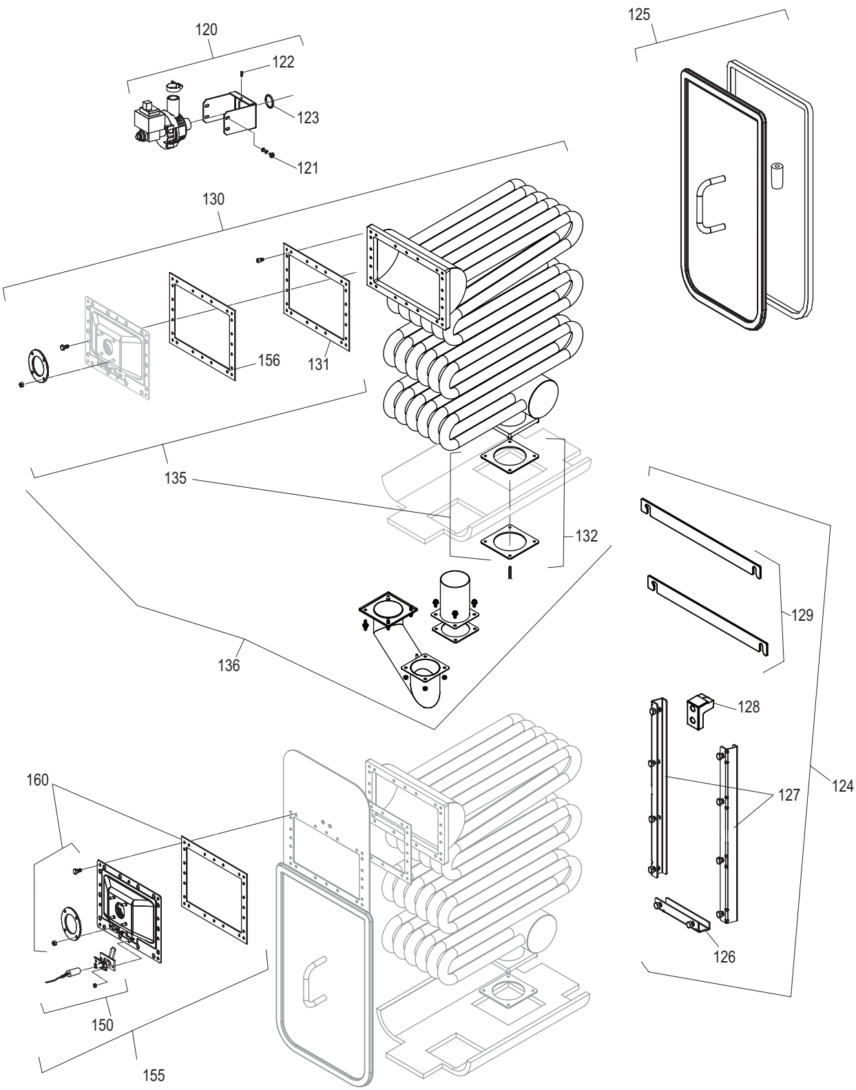
Figure 3: Nortec GS Humidifier, Kit Details Note: Greyed out items are not a part of the kits.
