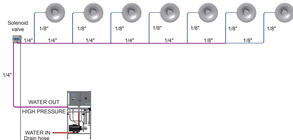
Figure 7: Hose layout inline
