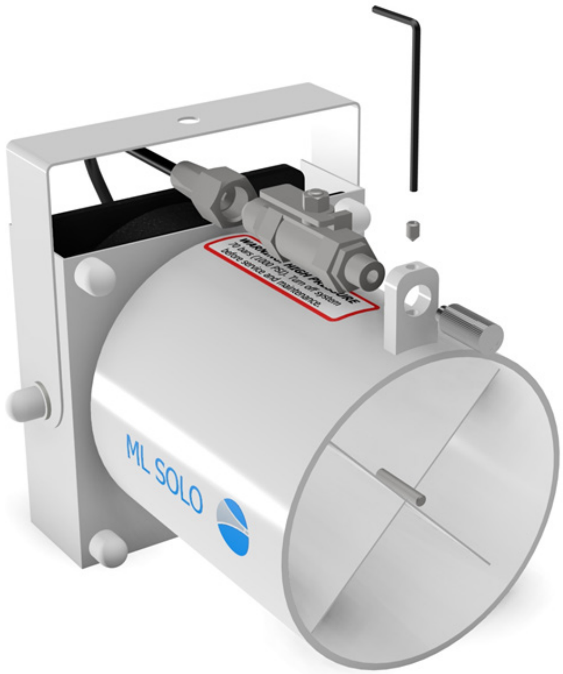
Figure 15: Assembling the ML Solo
