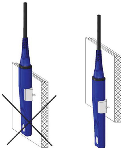
Figure 49: Mounting
