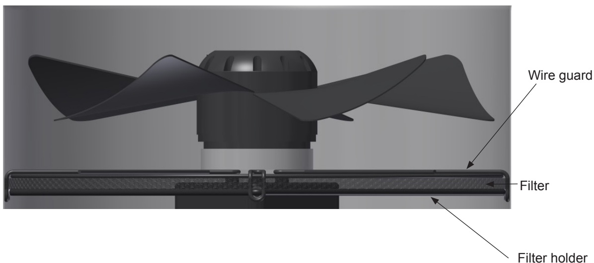
Figure 6: Filter assembly
